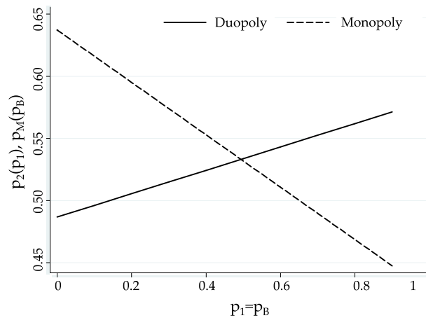
Fig. 3. Reaction functions p_2(p_1) and p_M(p) .
